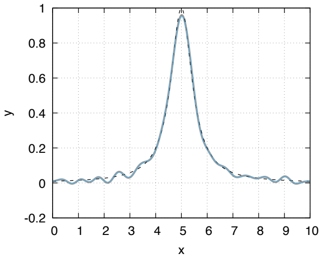
wiener filter applied to convolved bw signal
